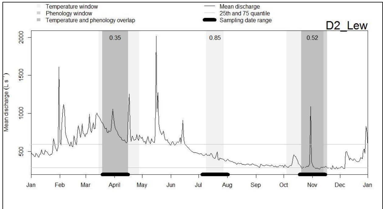
Figure 6. Proposed bouts for biological sampling at D02 Lewis Run. Sediment chemistry and fish sampling occur during Bouts 1 and 3.
