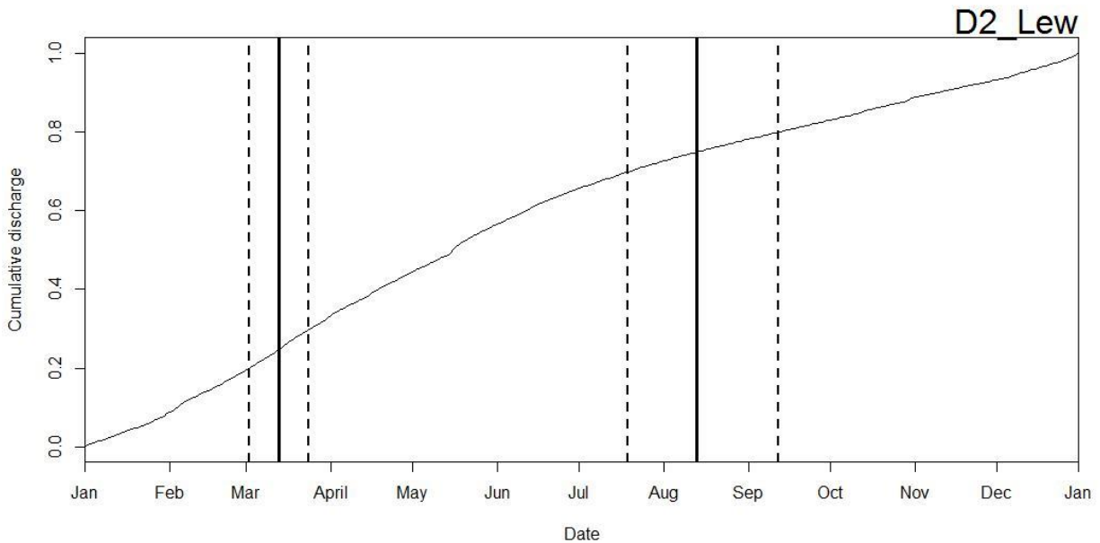
Figure 4. Timing of sample collection for 2 groundwater chemistry samples reflecting the discharge related strategy for Lewis Run.
