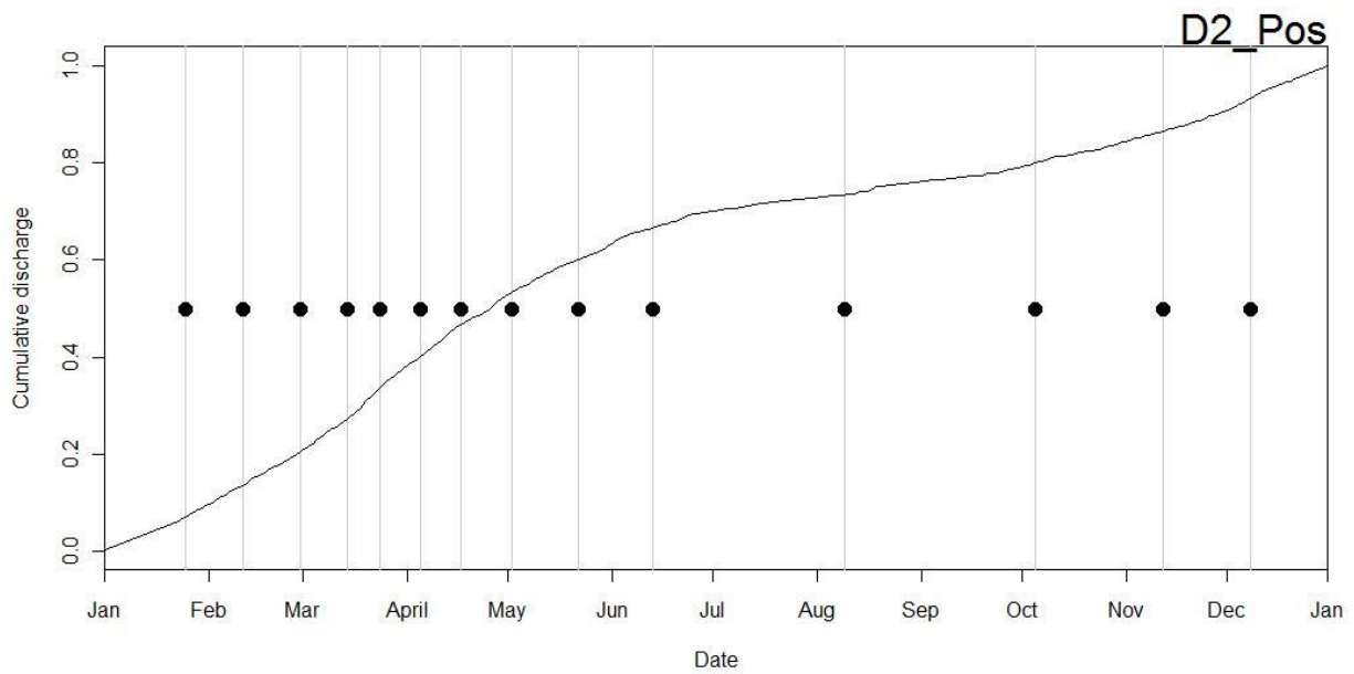
Figure 1. Timing of sample collection for 14 water chemistry samples reflecting the discharge related strategy for Posey Creek.
