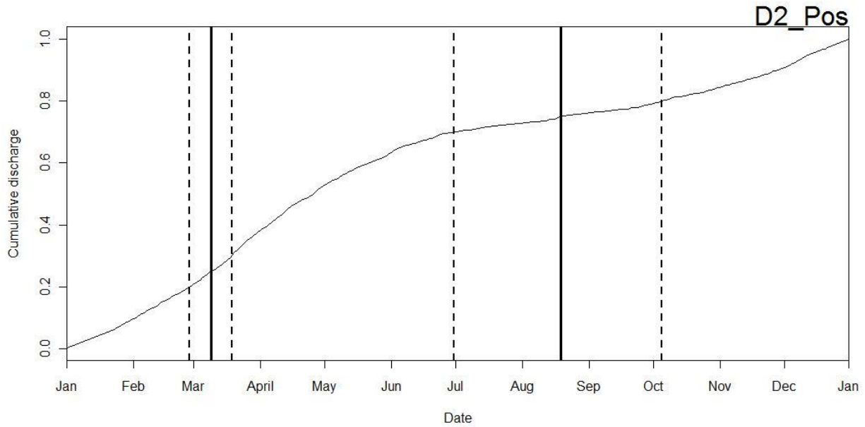
Figure 3. Timing of sample collection for 2 groundwater chemistry samples reflecting the discharge related strategy for Posey Creek.
