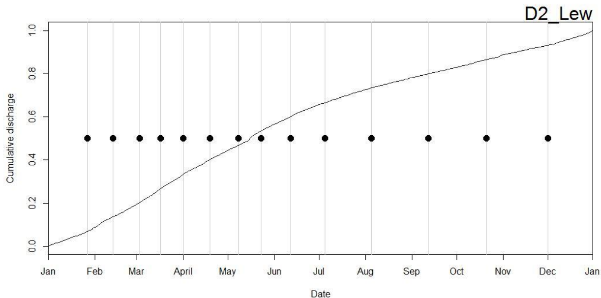
Figure 2. Timing of sample collection for 14 water chemistry samples reflecting the discharge related strategy for Lewis Run.
