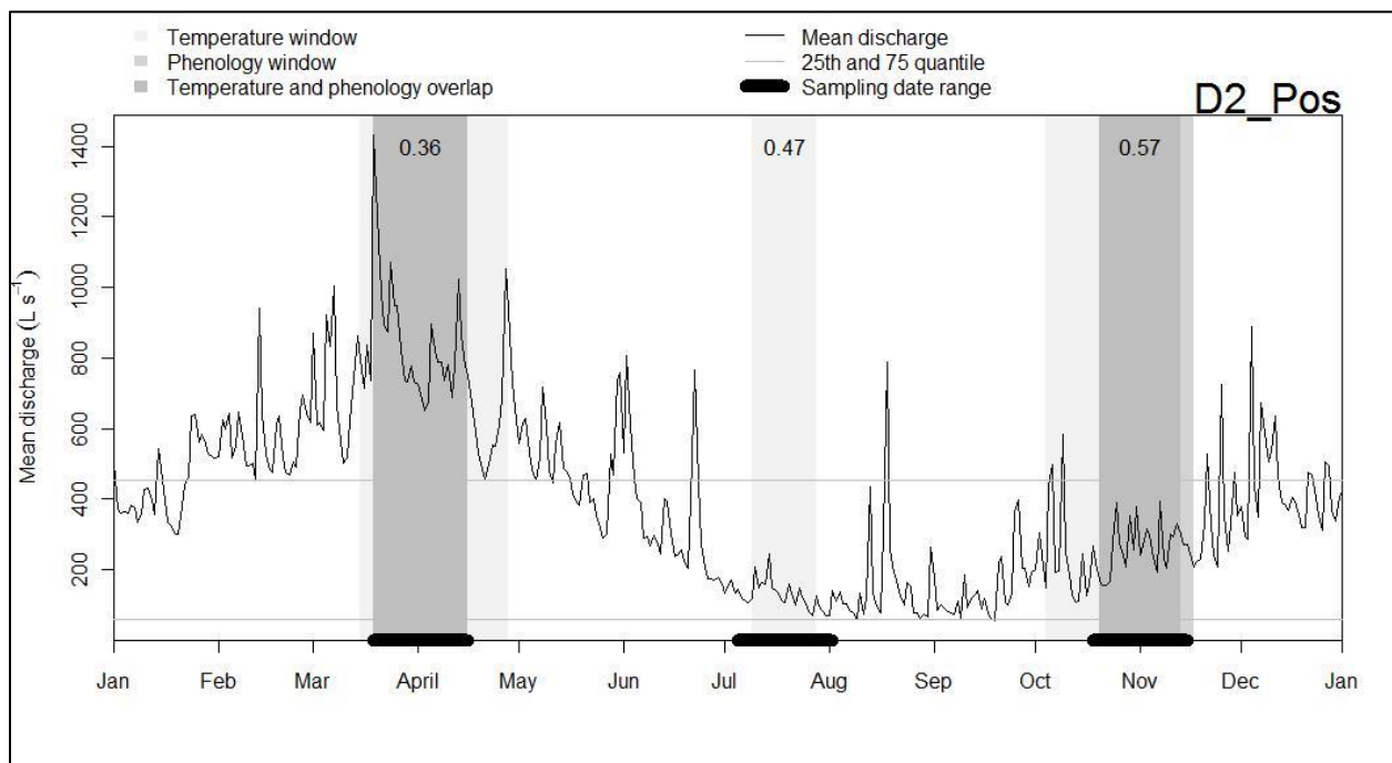
Figure 5. Proposed bouts for biological sampling at D02 Posey Creek. Sediment chemistry and fish sampling occur during Bouts 1 and 3.
