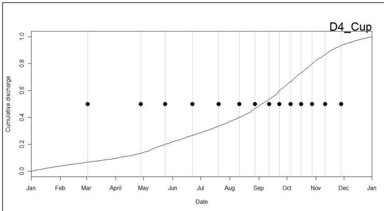
Figure 1. Timing of sample collection for 14 water chemistry samples reflecting the discharge related strategy for Rio Cupeyes.
