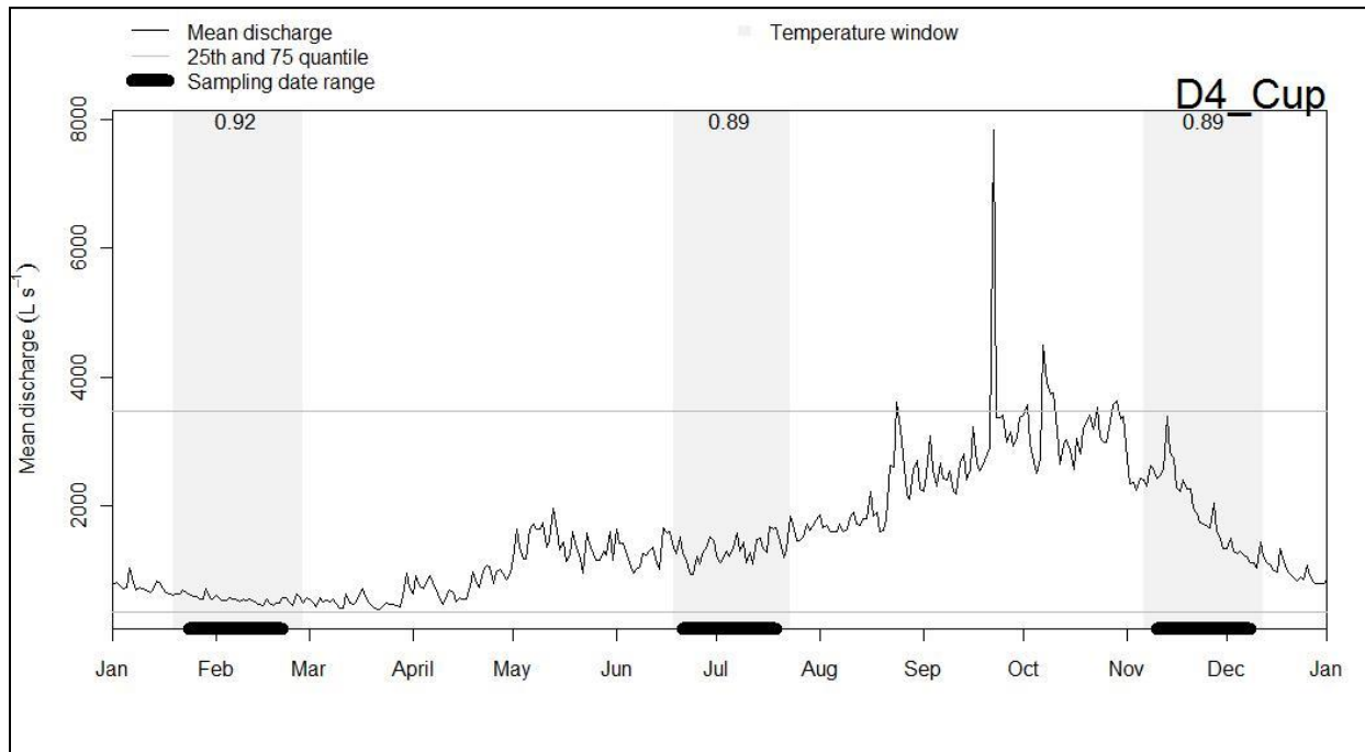
Figure 4. Proposed bouts for biological sampling at D04 Rio Cupeyes. Sediment chemistry and fish sampling occur during Bouts 1 and 3.
