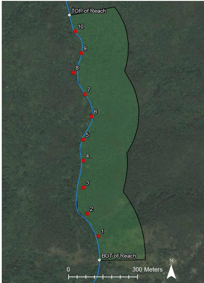
Figure 9. CUPE ideal riparian sampling design
