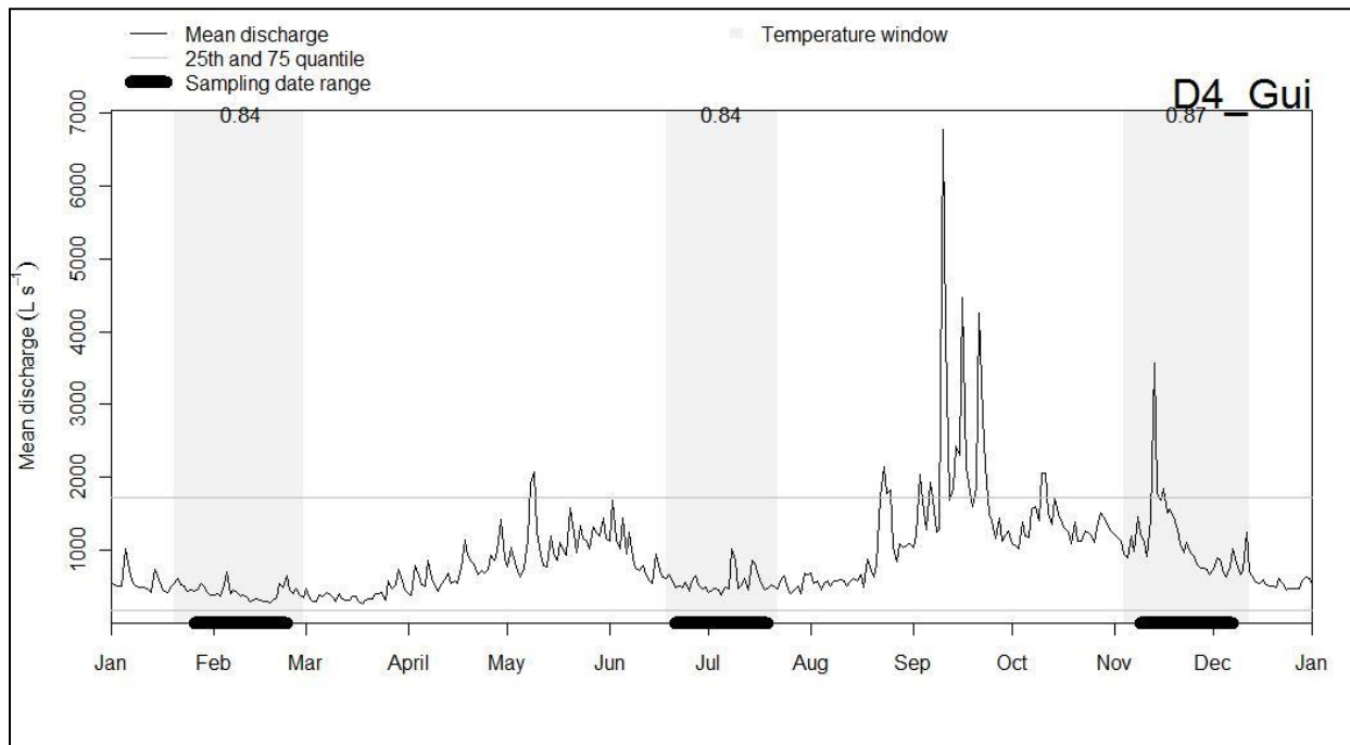
Figure 5. Proposed bouts for biological sampling D04 Rio Guilarte Sediment chemistry and fish sampling occurs during Bouts 1 and 3.
