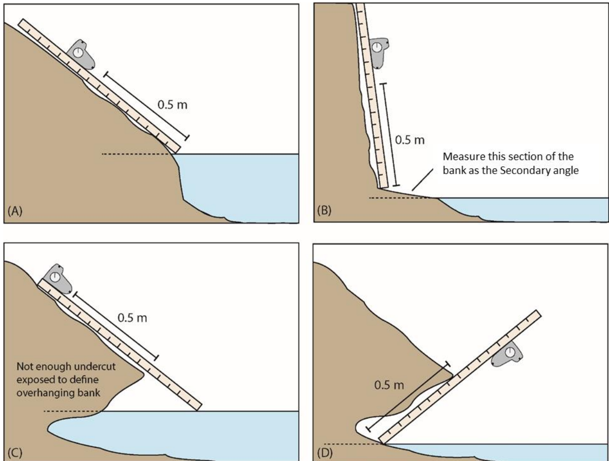
Figure 16. Bank angle using meter stick/clinometer. (A) Gradual shoreline (primary), (B) vertical bank (primary) incised channel (secondary), (C) gradual bank (primary) undercut stream
