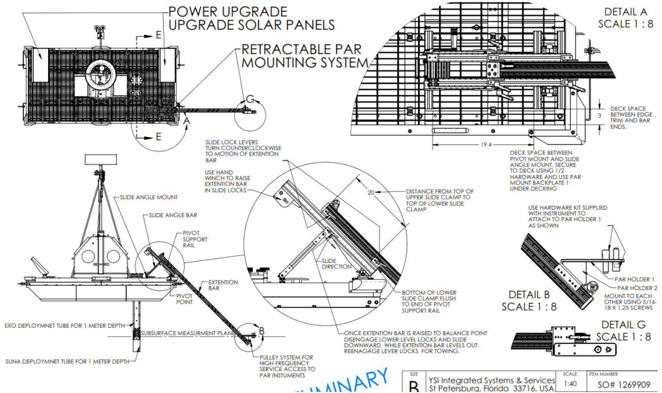
Figure 68. Retractable PAR Mounting System | FLNT River Buoy (Source: YSI Integrated Systems & Services) iv
