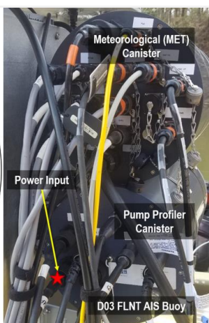
Figure 74. Pump Profiler Canister Port Mapping (Source: AD [13] )
