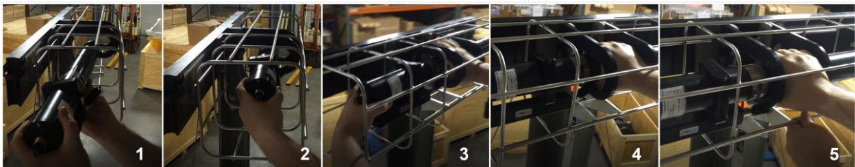
Figure 62. Reinstall SUNA from Dual PAR SUNA Mount Cage Clamps (Source: YSI Mechanical Engineer, Allen Hunter)
