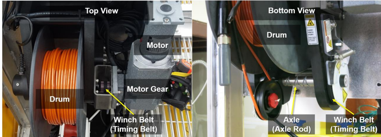
Figure 25. Winch Assembly Components
