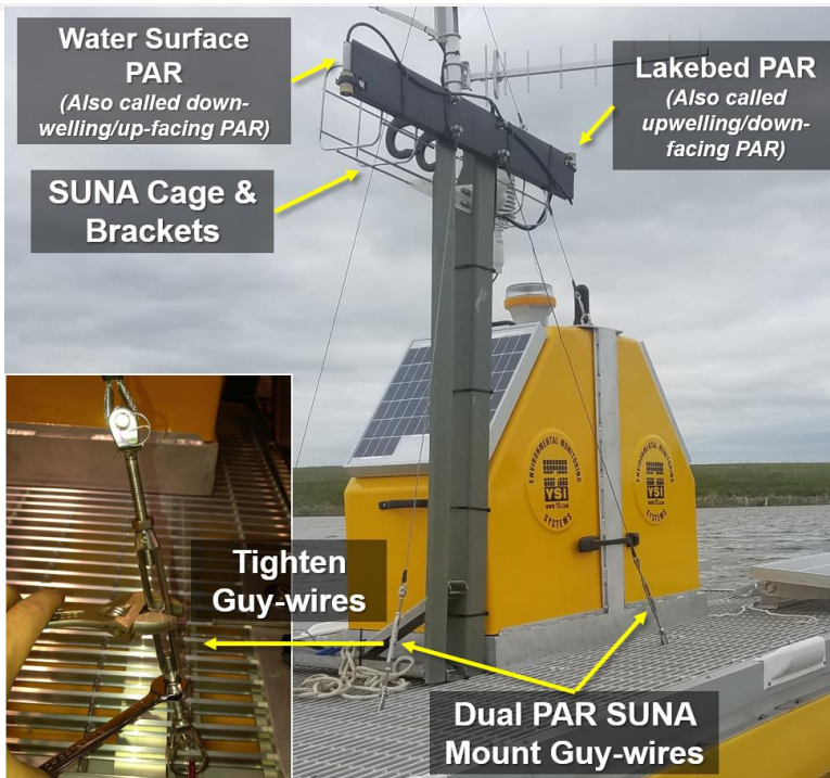
Figure 60. Raise the Dual PAR/SUNA Mount on the AIS Buoy
