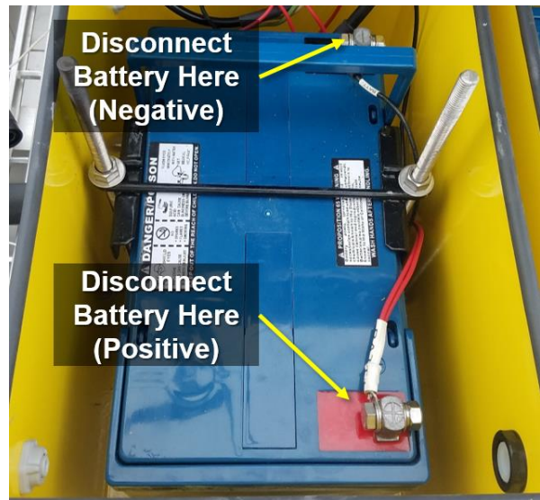
Figure 38. Disconnect the Batteries to Remove from the Battery Enclosure
