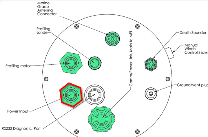
Figure 59. Profile Canister Port Mapping (Source: AD [13] )
