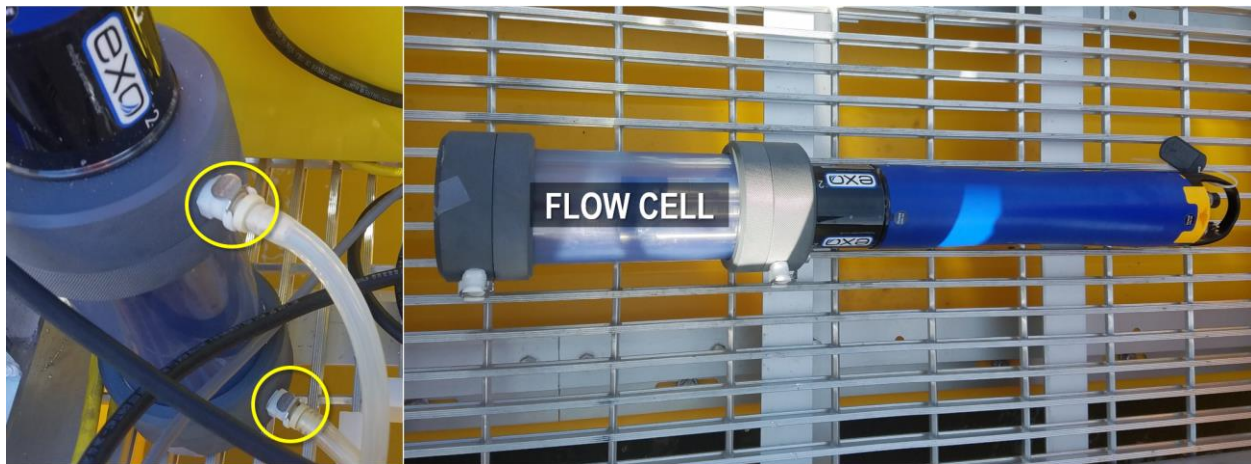
Figure 56. Remove Multisonde from Flow Cell
