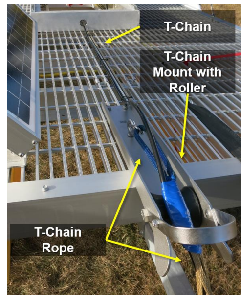
Figure 23. T-Chain and T-Chain Mount on Floating Deck
