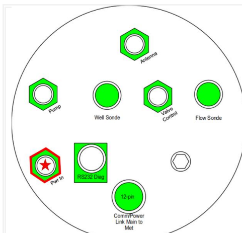
Figure 74. Pump Profiler Canister Port Mapping (Source: AD [13] )
