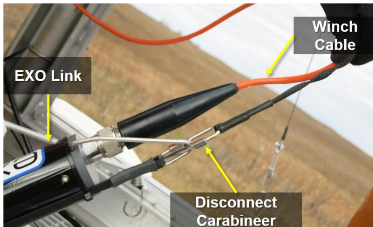
Figure 50. Disconnect Multisonde from the Lake Buoy Winch
