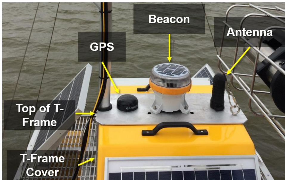
Figure 14. T-Frame: GPS, Beacon and Antenna
