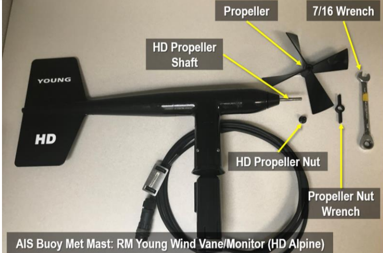
Figure 91. RM Young Wind Vane Propeller Parts/Equipment for Removal
