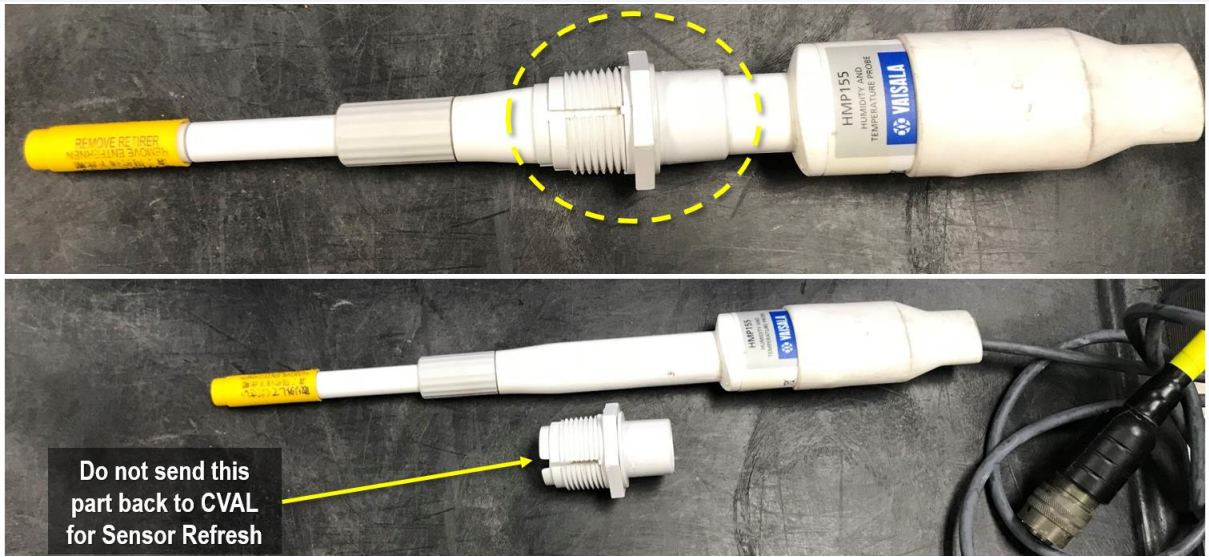
Figure 94. Vaisala HMP-155 Sensor with Yellow Protective Cap & Radiation Shield Mounting Component – Do Not Send to CVAL
