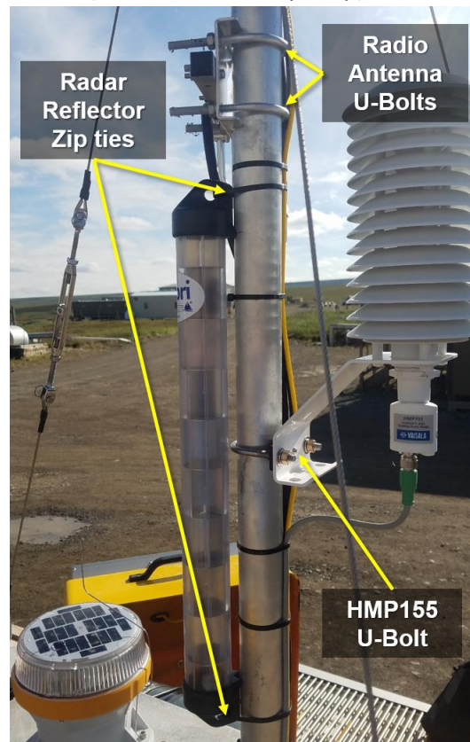
Figure 40. Remove Instruments from Met Mast
