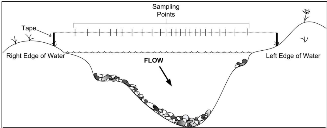
Figure 3. Uneven subsections across sampling transect
