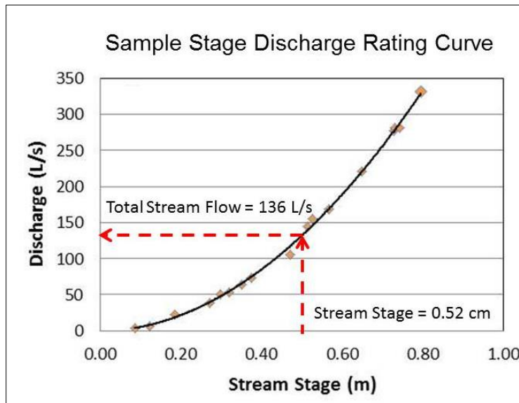
Figure 9. Example of stage-discharge rating curve. Dots represent simultaneous measurements of stage and discharge
