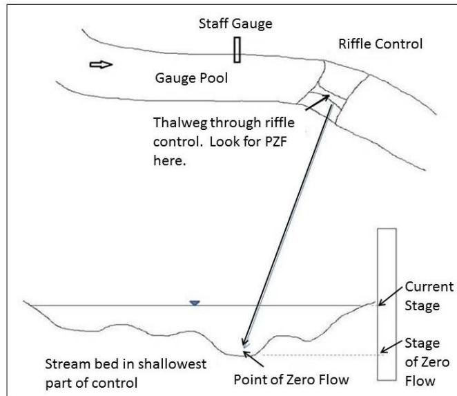
Figure 8. Diagram showing point of zero flow and stage of zero flow
