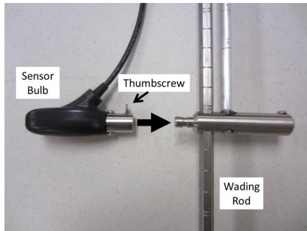
Figure 5. Velocity-meter and the thumbscrew that attaches it to the wading rod
