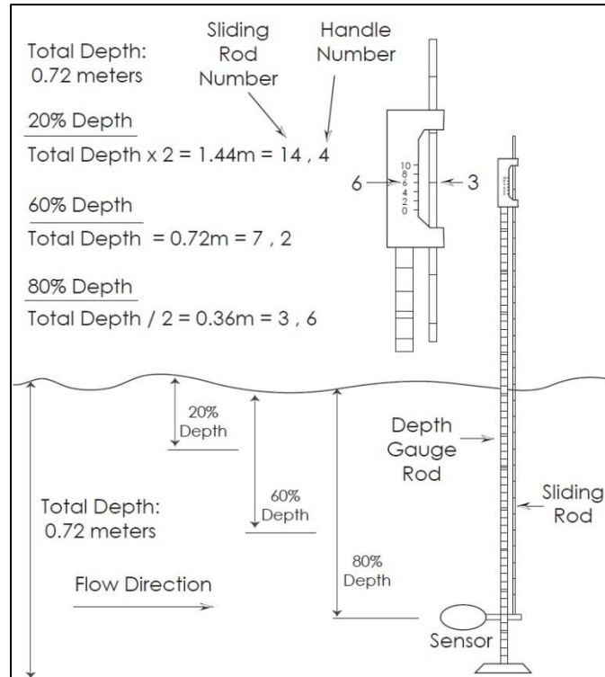
Figure 4. Correctly-assembled wading rod adjusted to 80%
