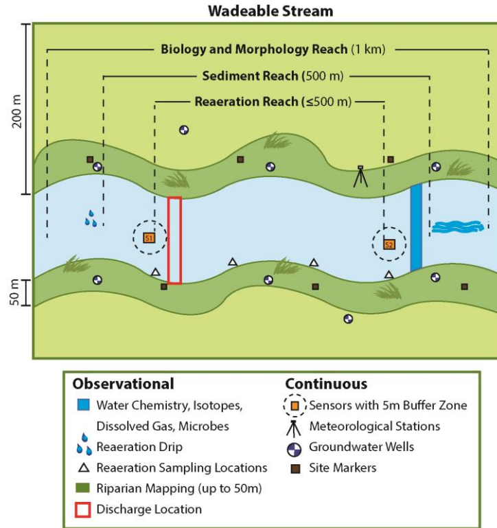
Figure 1. A generic wadeable stream site with the discharge sampling location
