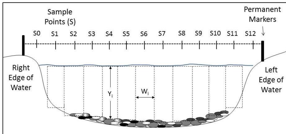
Figure 2. Example of an excellent distribution of measurement sections
