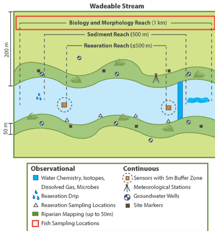
Figure 3. A generic wadeable stream site layout with fish sampling locations
