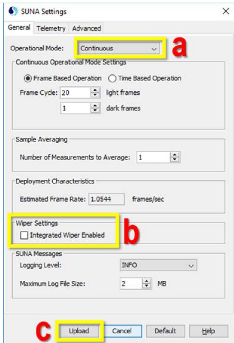
Figure 30. Configure SUNA for Validation Process
