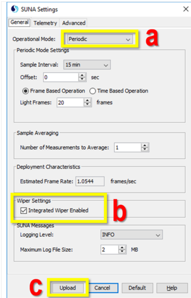
Figure 45. Return SUNA to Original Settings for Deployment
