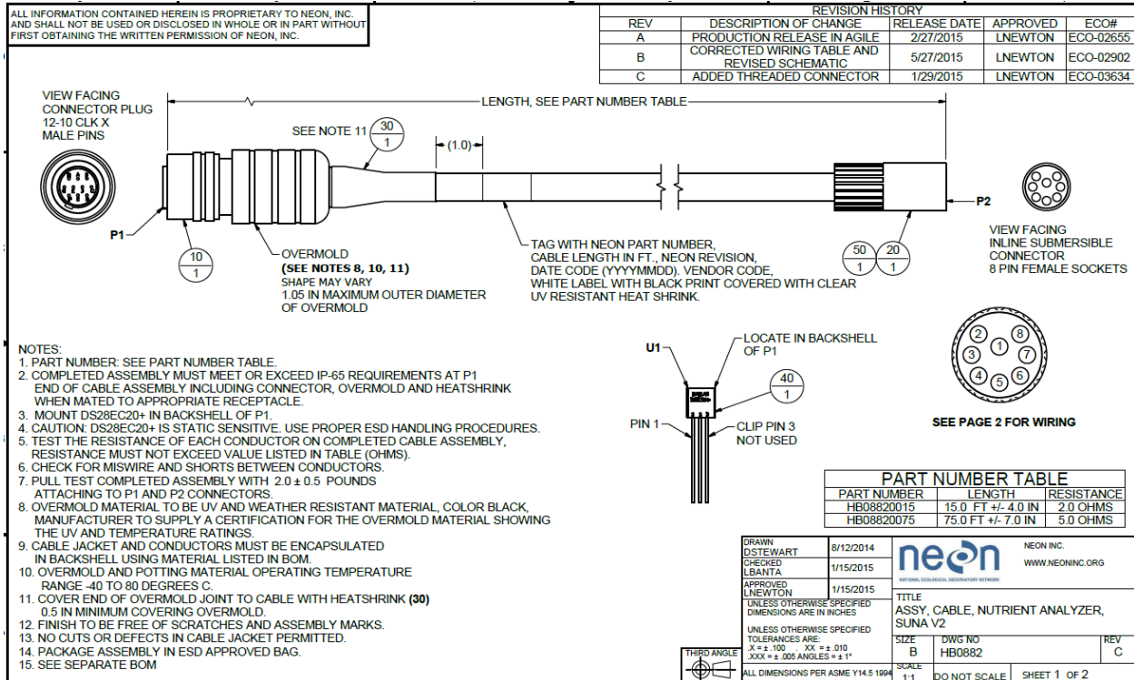
Figure 82. SUNA Power Cable Drawing.
