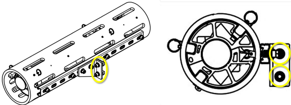
Figure 70. Remove the 2 Bolts that Attach the Mount
