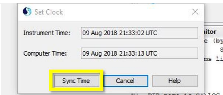
Figure 48. Select "Sync Time" to Automatically Update the SUNA Clock
