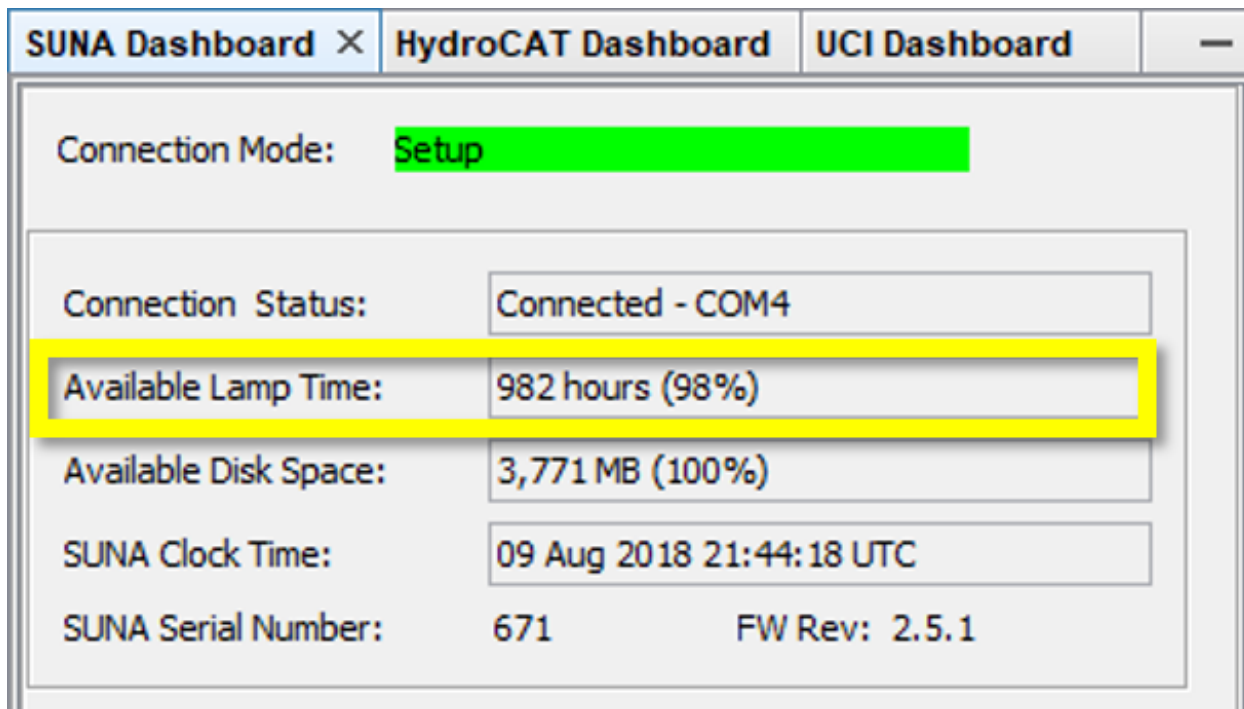
Figure 46. SUNA Dashboard: Available Lamp Time | Verify Lamp Time is > 50 Hours.
