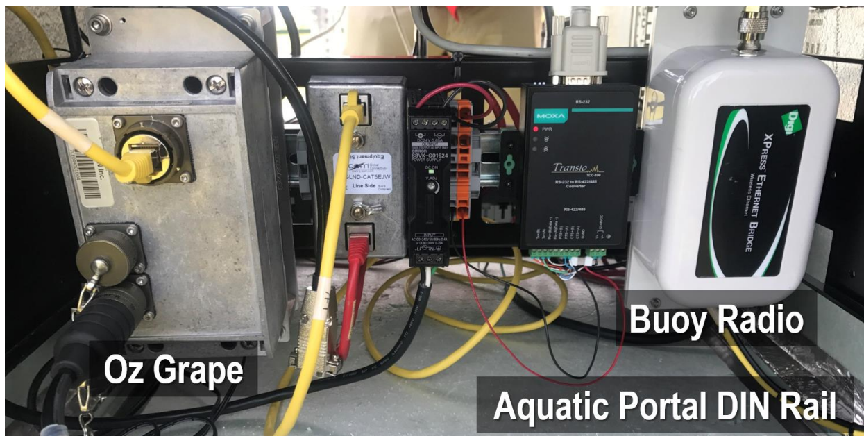
Figure 8. Aquatic Portal Precip DIN Rail: AIS Buoy Portal Radio/Oz Grape Subsystem.
