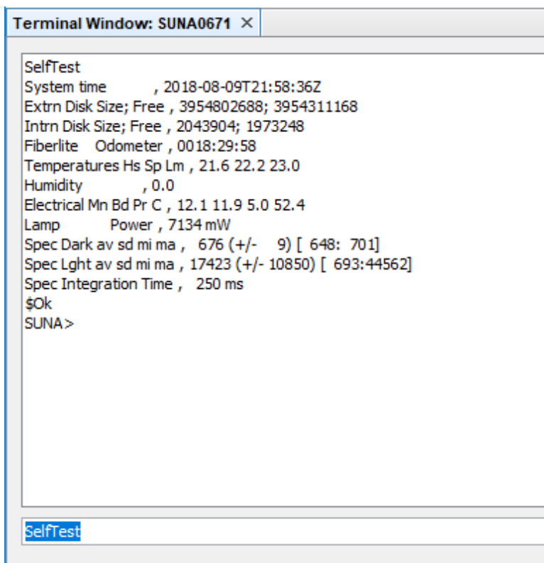
Figure 54. "SelfTest" Output Populates in the Terminal Window
