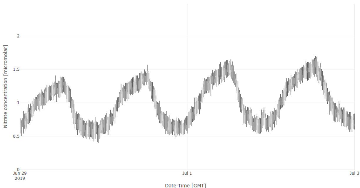
Figure 84. This is an example of what good SUNA data looks like. Each line represents a 15 burst. Check that there are data every 15 minutes. Note the low variance within burst and low variance from one burst to the next. You can view individual values by zooming in and hovering the cursor over them. This site shows diel variation in nitrate produced by processes such as plants assimilating nitrate and microbes performing denitrification. Diel variation is a common (but not ubiquitous) feature of aquatic nitrate signals.
