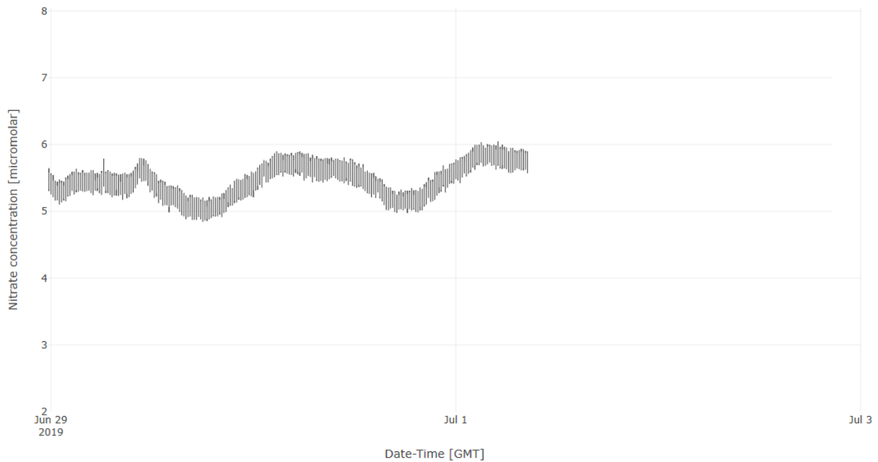
Figure 91. This example shows the SUNA was transmitting quality data until a PM occurred, at which point it stopped streaming. Check that UCI was exited out of correctly (5.5 Step 2), re-open and disconnected correctly if needed. Check that the SUNA cable was reconnected to the Grape data logger. Check that the SUNA was acquired by the Grape (5.5 Step 5); power cycle the Grape, if necessary.
