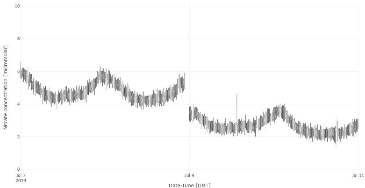
Figure 86. This is an example of how PM such as cleaning or calibration can affect the nitrate concentration. Biofouling on the lens or reduction in lamp output causes less light to reach the SUNA detector. The SUNA assumes this is happening because more light is being absorbed by nitrate, and so it predicts a higher concentration. Cleaning and reference updates will usually cause the concentration to drop. The change in the concentration measured in water should be comparable in magnitude to the change measured in DI as part of the PM.
