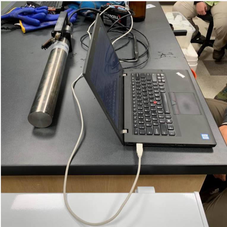
Figure 24. Example of Complete Setup for SUNA Validations
