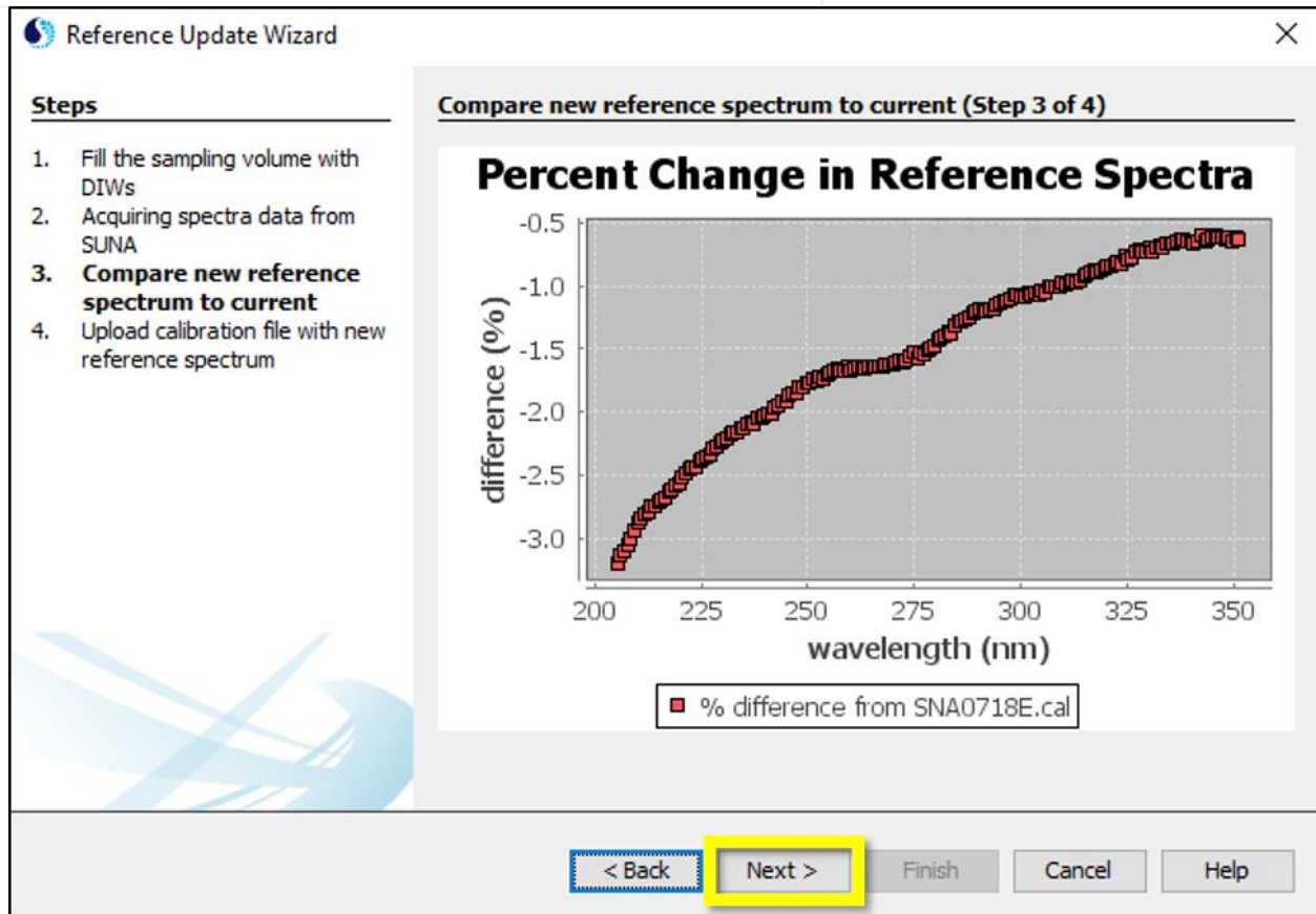
Figure 60. Reference Update Wizard Step 3 of 4: Compare New Reference Spectrum to Current
