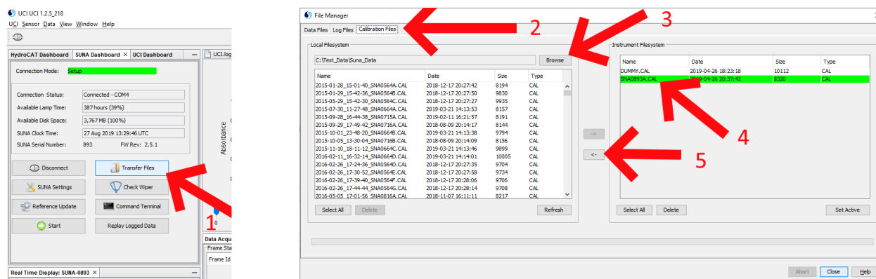
Figure 84. Process to Manually Download SUNA Calibration Files.
