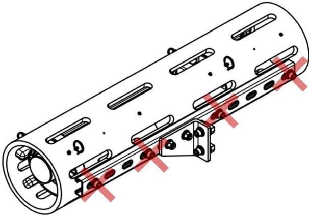
Figure 71. Do Not Remove these 4 Bolts
