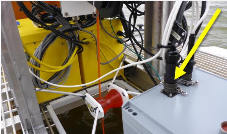
Figure 22. Attach Y-Cable to SUNA Radio Box at Buoy Sites
