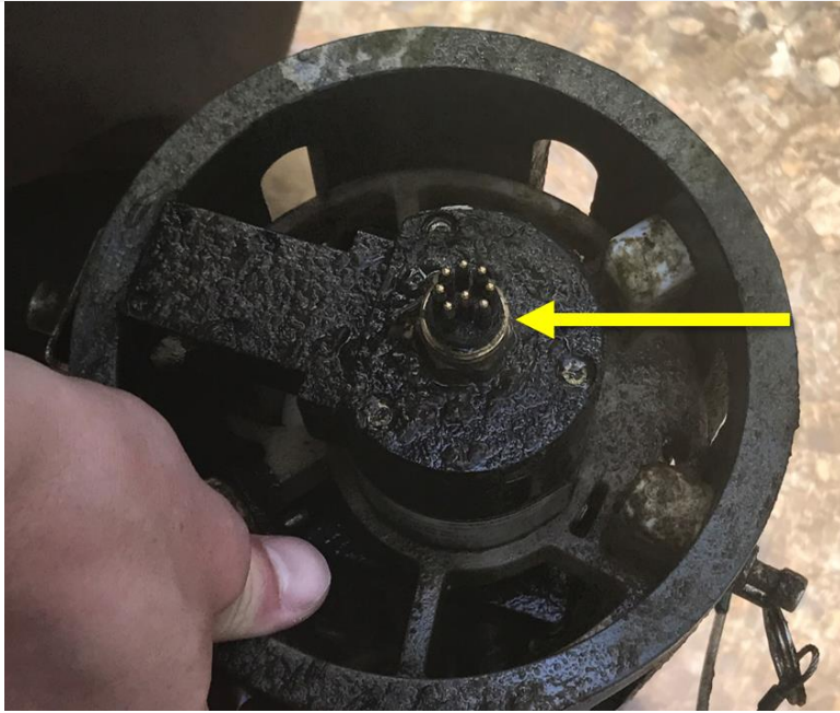
Figure 16. SUNA Bulkhead Connector
