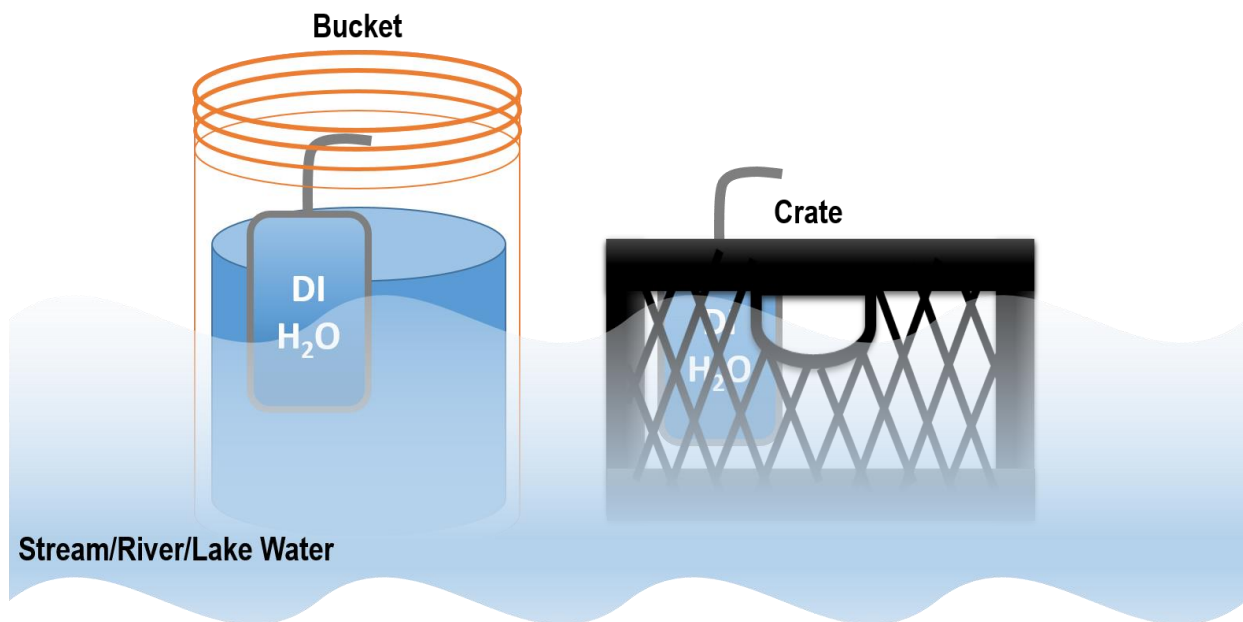
Figure 12. Alternate Setups for DI Water Temperature Equilibration .
