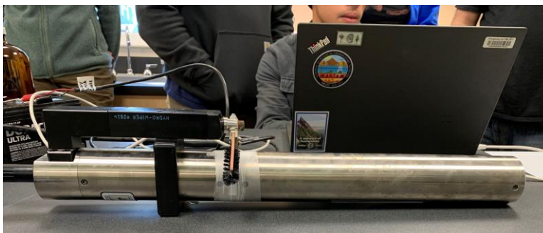
Figure 35. Validate SUNA Vertically to Prevent Bubbles on Optical Bench
