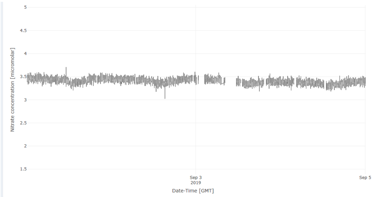
Figure 90. This example shows otherwise good data with gaps in it. This is usually a communication issue, not a sensor issue. Check the connection between the SUNA and the Grape data logger. For buoy sites, check the radio link. This particular example occurred for a buoy whose moorings were lose allowing wind to rotate the SUNA antenna out of line of sight with the shore receiver.
