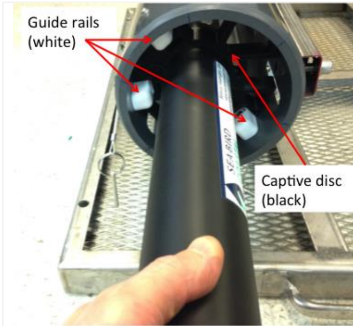
Figure 75. Remove Sensor from PVC Enclosure
