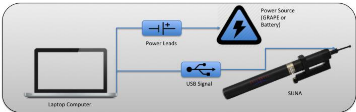
Figure 20. Functional Diagram of Y-Cable Connections for Validation Process
