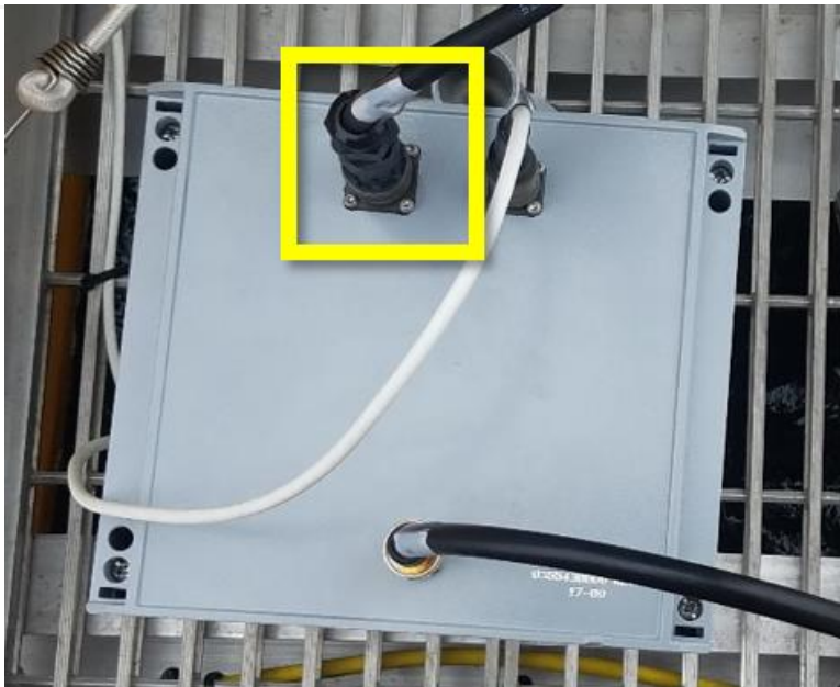
Figure 15. SUNA Radio Box on AIS Buoy: Power Connector (12-10)
