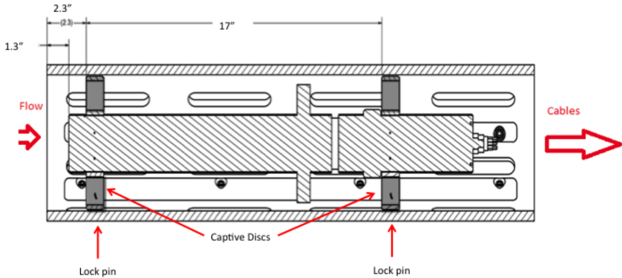
Figure 73. SUNA Orientation and Installation Components
