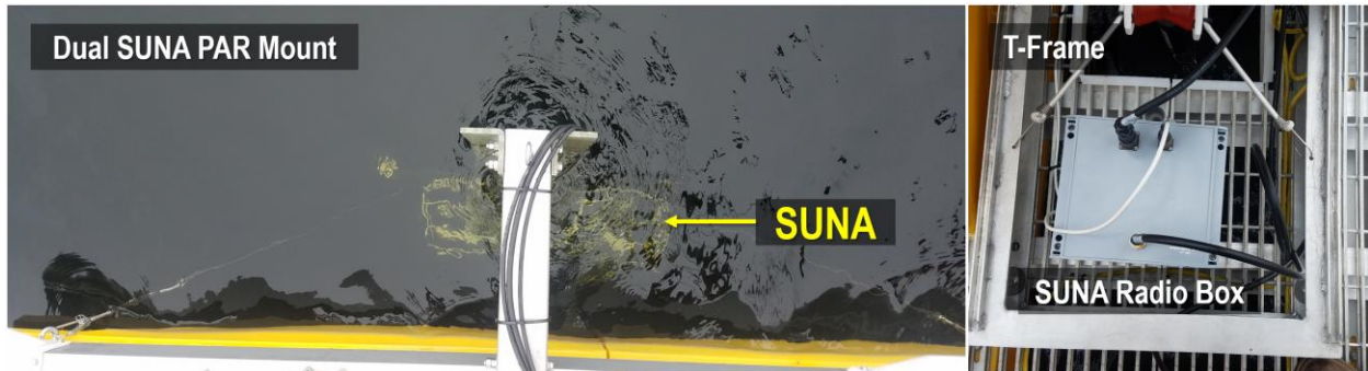
Figure 6. Dual SUNA PAR Mount and Radio Box on AIS Buoy
