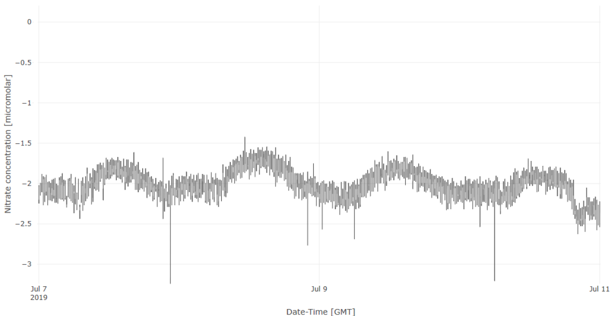
Figure 87. This example shows data with low variance and diel variation, but the concentrations are negative. The reference spectrum may have been calibrated incorrectly (the lens was not clean or DI was contaminated). Re-perform the update. If the problem persists the SUNA needs to be serviced.
