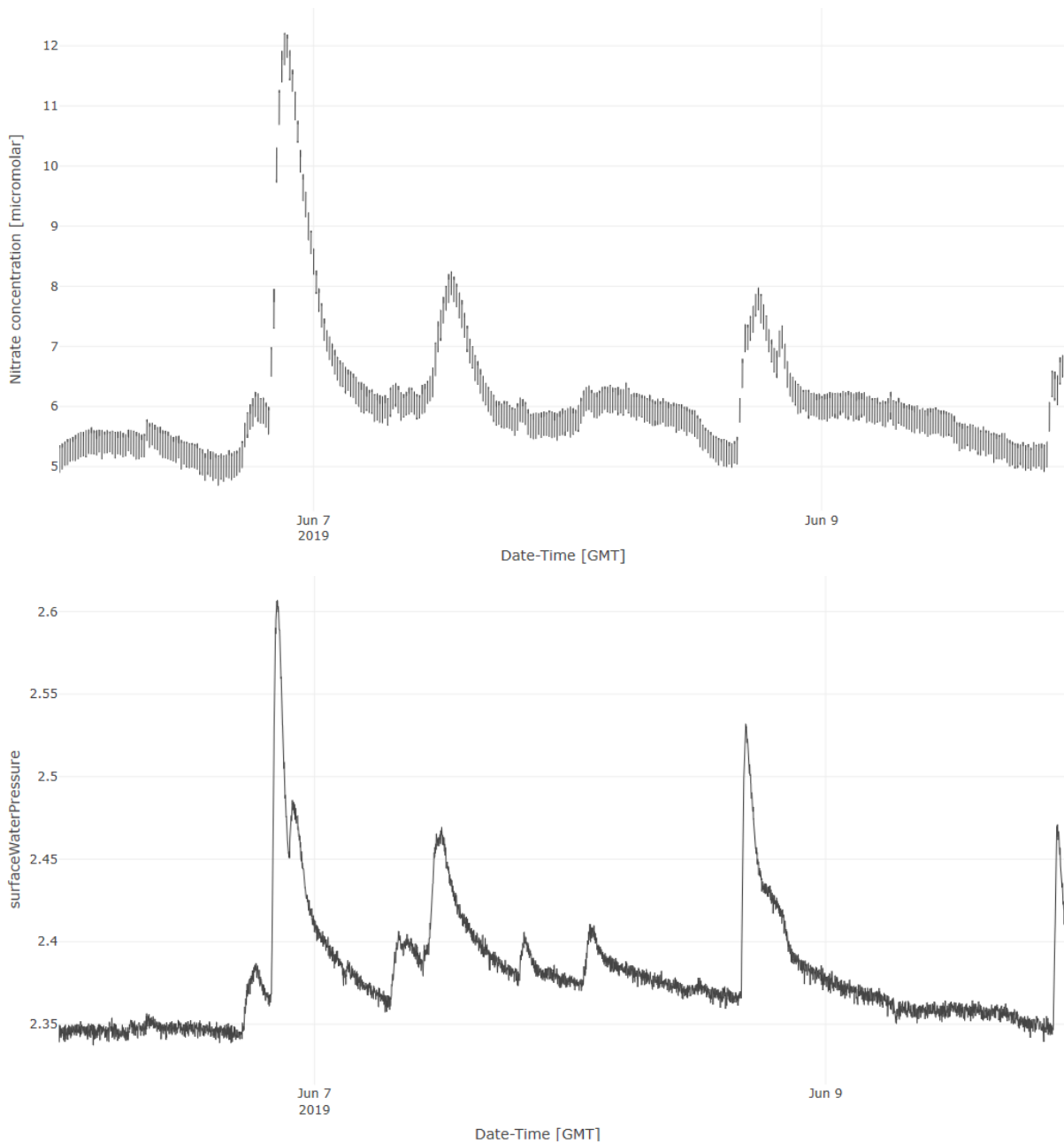
Figure 85. This is an example shows large and rapid spikes in nitrate concentration. However, if we also look at the water surface pressure data on Blizzard, we can see that there were contemporaneous increases in water depth, suggesting storm events occurred. Storm events can enrich or dilute nitrate concentrations, producing sudden peaks or troughs. This is normal. However, sudden and large nitrate peaks without a change in water level or other chemical parameters (check the Multisonde data) it can be cause for concern. If you see unusual behavior in the nitrate data, check and see if it also occurs in other data streams, which might indicate it is natural variation.
