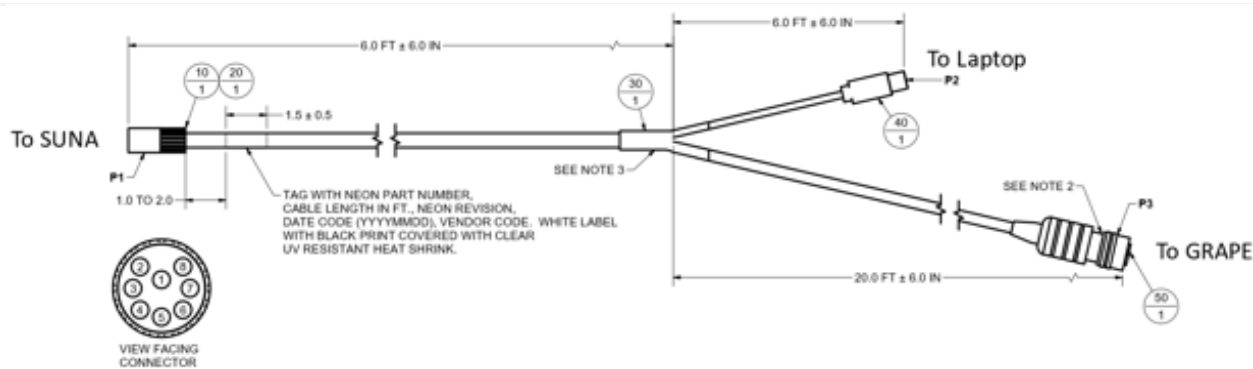
Figure 13. NEON Custom Y-Cable for Stream, Lake and River SUNA Field Validations/Calibrations (HB09780000)
