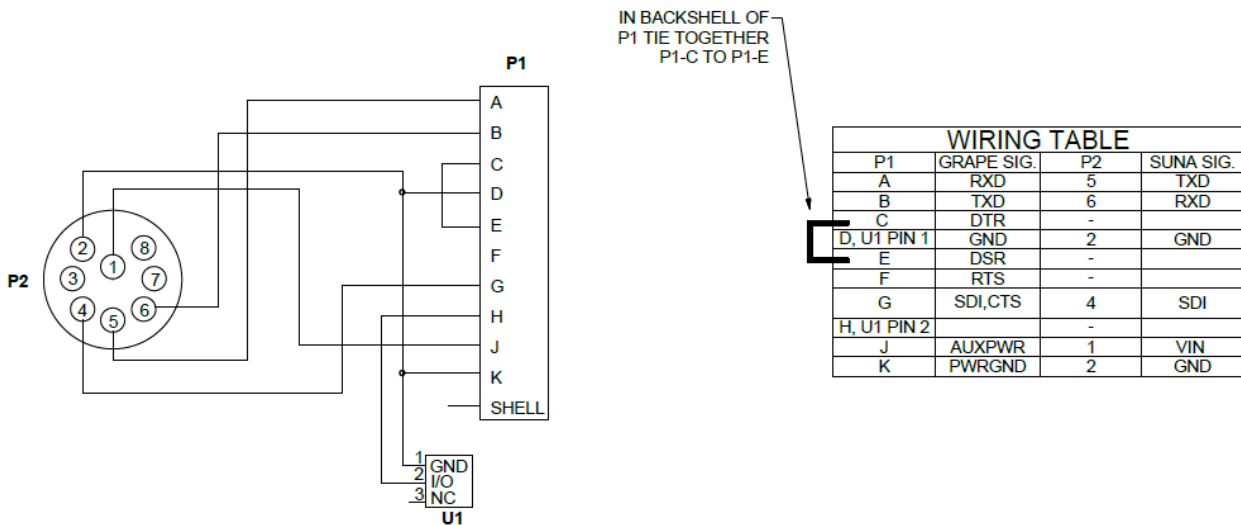
Figure 83. SUNA Power Cable Wiring.
