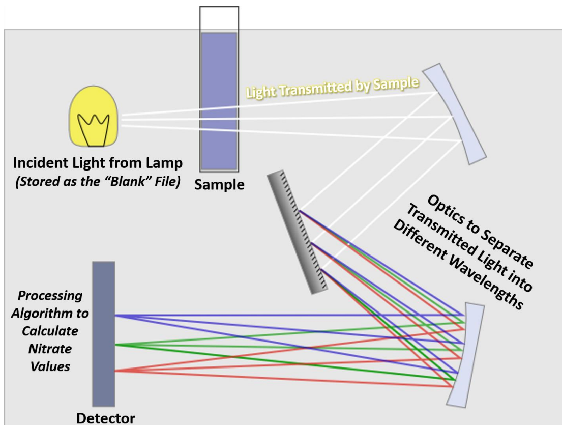
Figure 2. Overview of How a Spectrometer, such as the SUNA, Creates Absorbance Measurements.
