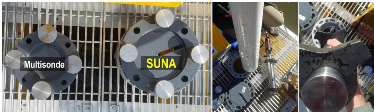
Figure 7. SUNA Location on AIS Buoy for D03, FLNT.
