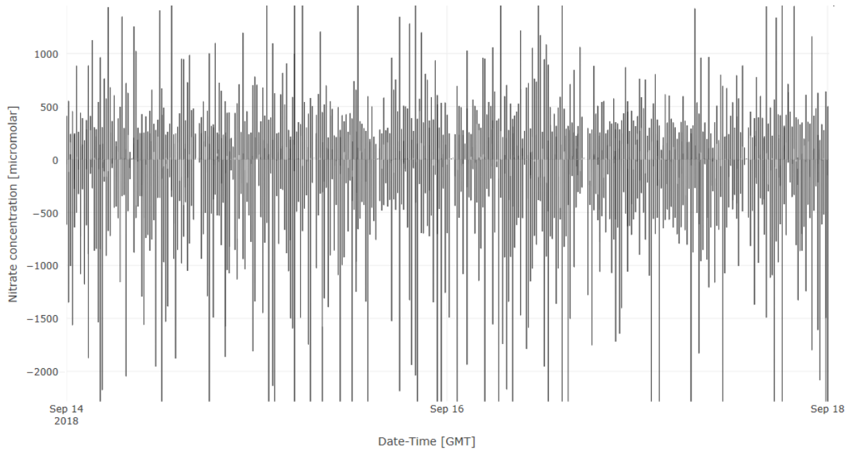
Figure 88. This example shows data with large variance both within and across bursts. The sensor is potentially fouled or the lamp has degraded. Check that the sensor is not buried, clean the optical lens, perform a reference spectrum update and then a self-test to measure the lamp output.
