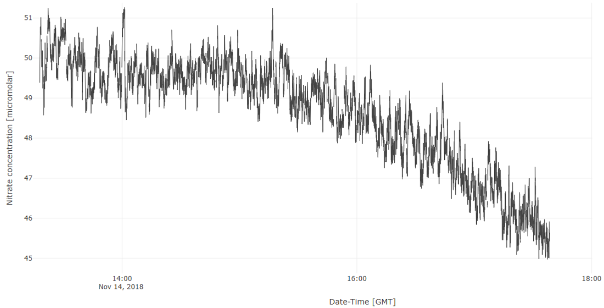
Figure 90. This example shows continuous data rather than 15 minute bursts. The SUNA was accidentally left in Continuous mode following PM. Reconnect to the SUNA and correct the settings to Periodic.
