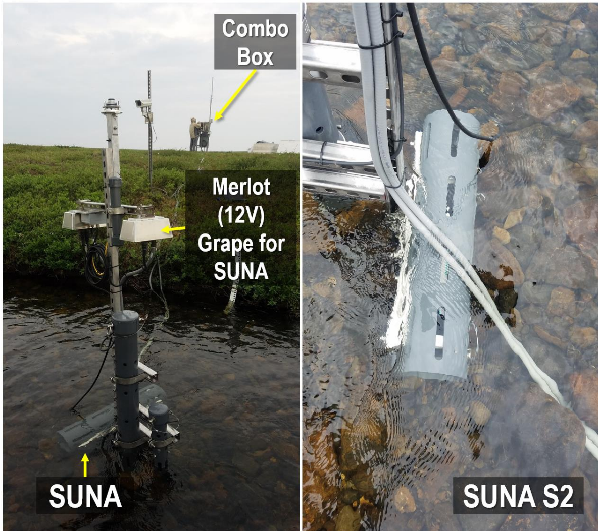
Figure 3. S2 Downstream Location: SUNA on an Anchor with Subsystem Components at a Low Water Site.
