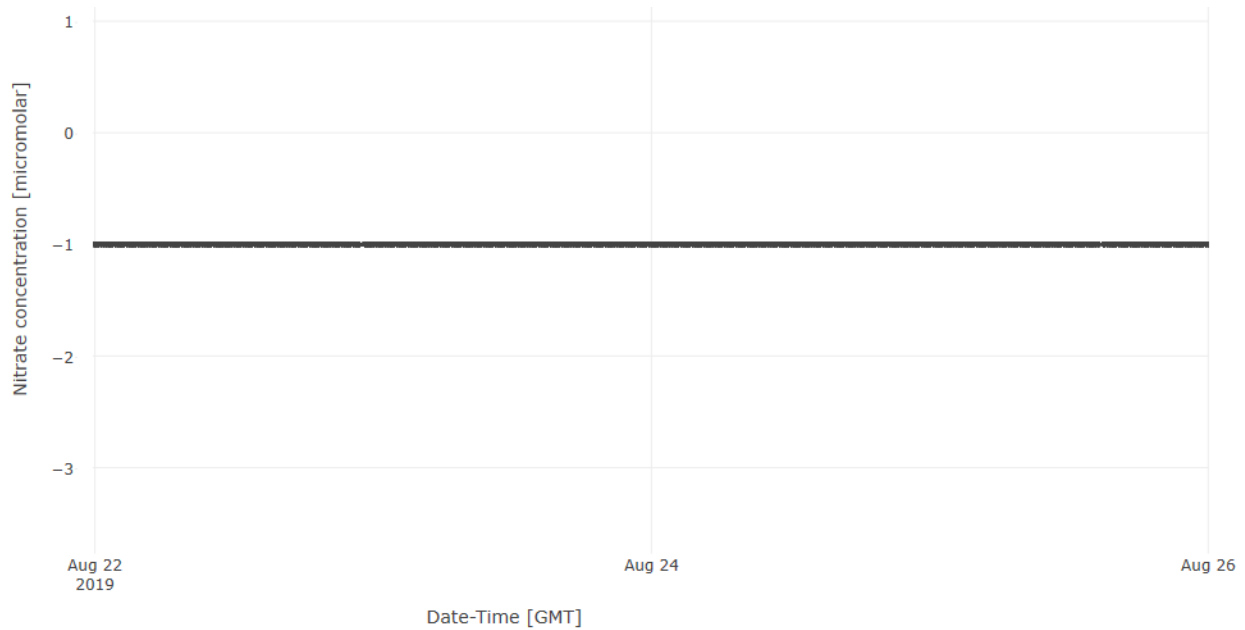
Figure 89. This example shows a string of all “-1”. This is not a real concentration, but an error code the SUNA uses to report low transmittance. Report to Aquatic Science Team.
