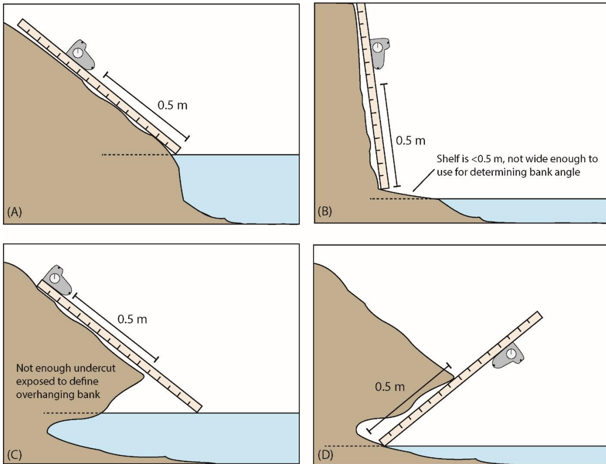
Figure 11. Determining shoreline bank angle for different bank types using a meter stick and clinometer. (A) Gradual shoreline, (B) incised channel with a vertical bank angle, (C) gradual bank with an undercut stream bank, and (D) overhanging stream bank.
