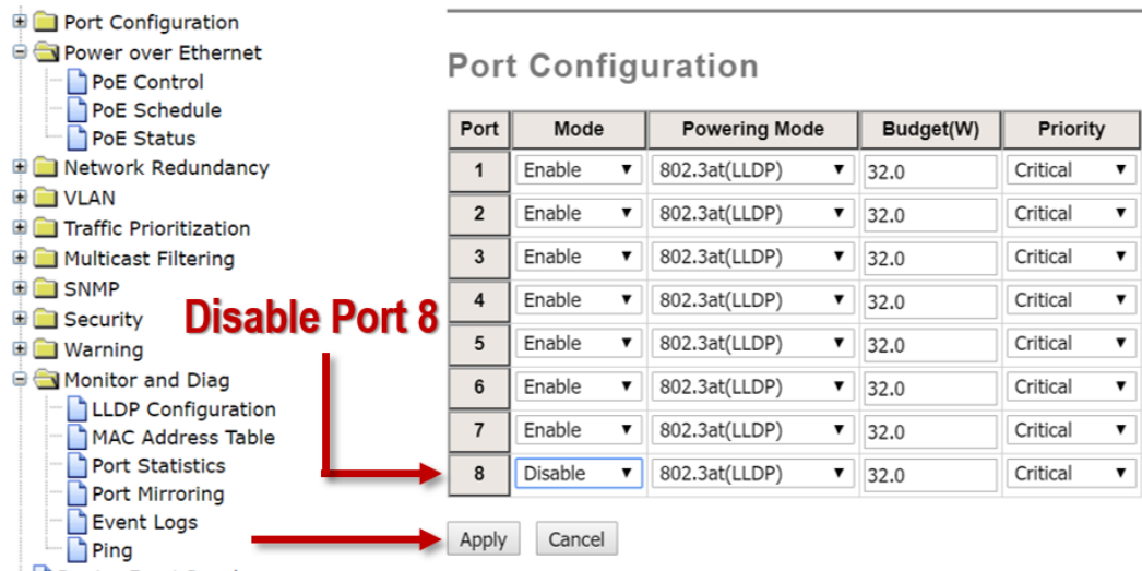
Figure 69. PoE Switch Port Configuration
