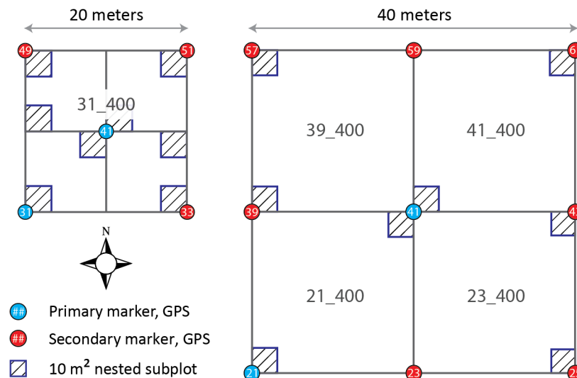
Figure 2: Plot, subplot and nested subplot layout in 20mx20m and 40mx40m Tower plots
