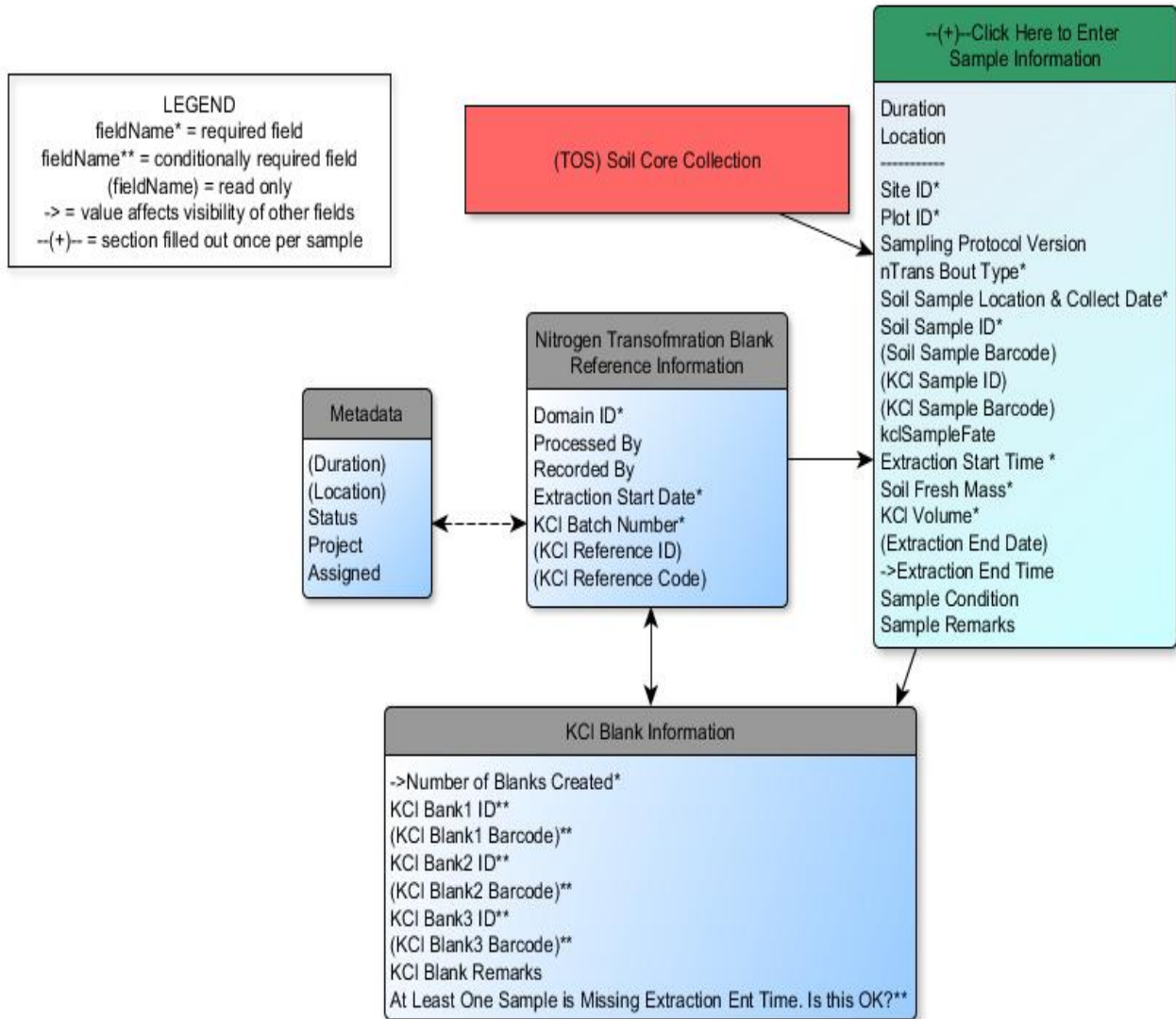
Figure 3: Schematic of the application used by field technicians to enter KCI extraction data
