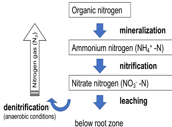
Figure 1: Simple overview diagram of the nitrogen cycle. Reproduced from University of California Cooperative Extension.
