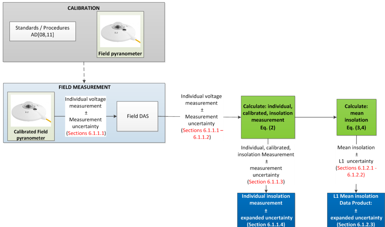
Figure 2: Displays the data flow and associated uncertainties of individual insolation measurements and L1 insolation DPs. For a detailed explanation of pyranometer calibration procedures, please refer to AD[08,11].
