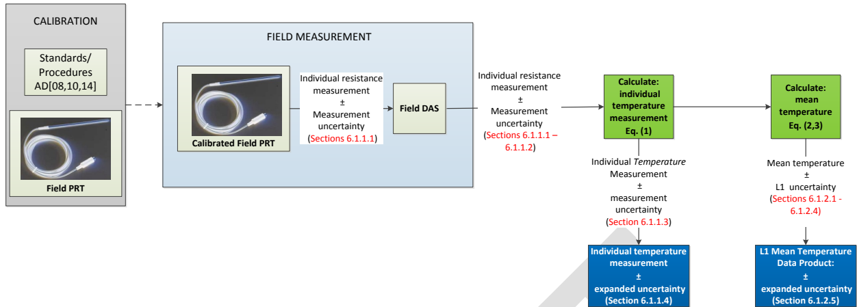
Figure 2: Displays the data flow and associated uncertainties of individual temperature measurements and L1 mean soil temperature DPs. A detailed explanation of the PRT calibration procedures, please refer to AD[08,10,14].
