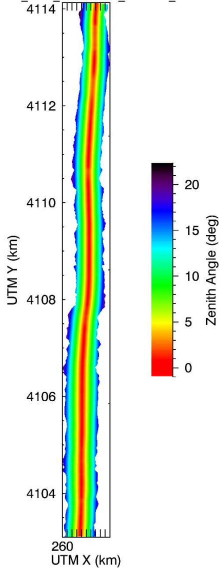
Figure 3 - False color image of the LOS zenith angle at the ground for the image NEON_D17_SJER_DP1_20170328_174440_reflectance.h5
