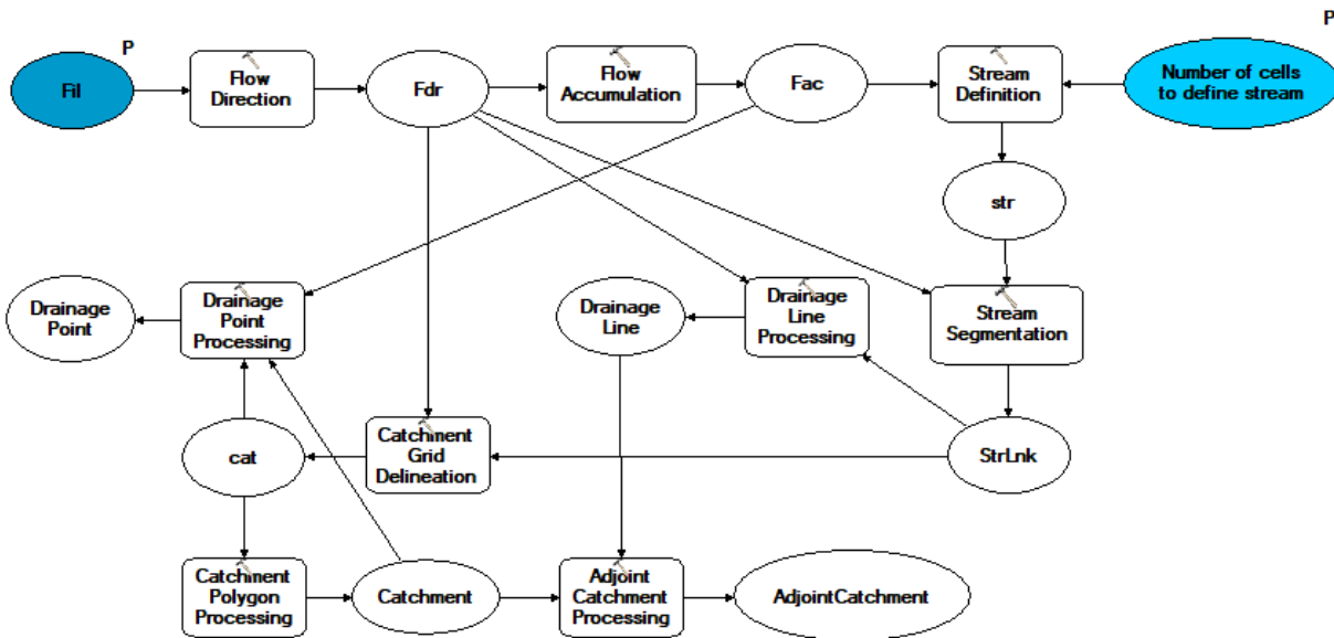
Figure 1 - Basic Dendritic Terrain Processing Model
