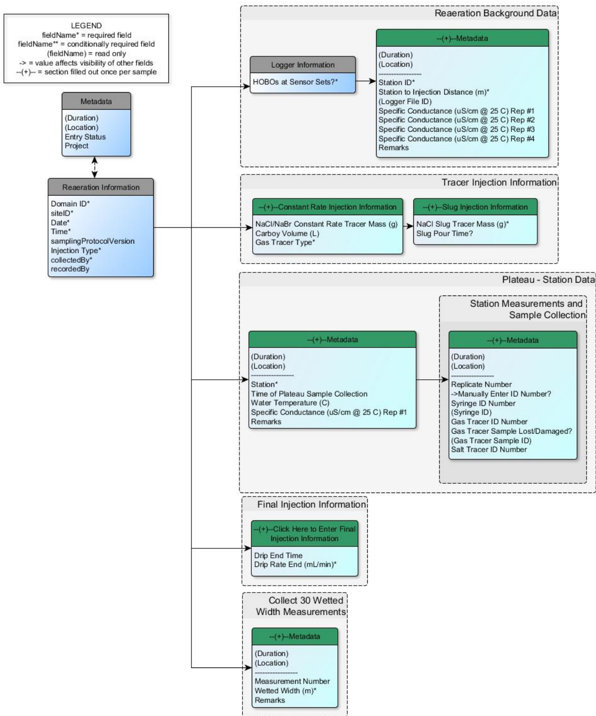
Figure 2: Schematic of the applications used by field technicians to enter reaeration and salt-based discharge data
